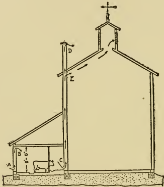
Sketch B—Method of ventilating a lean-to stable.
